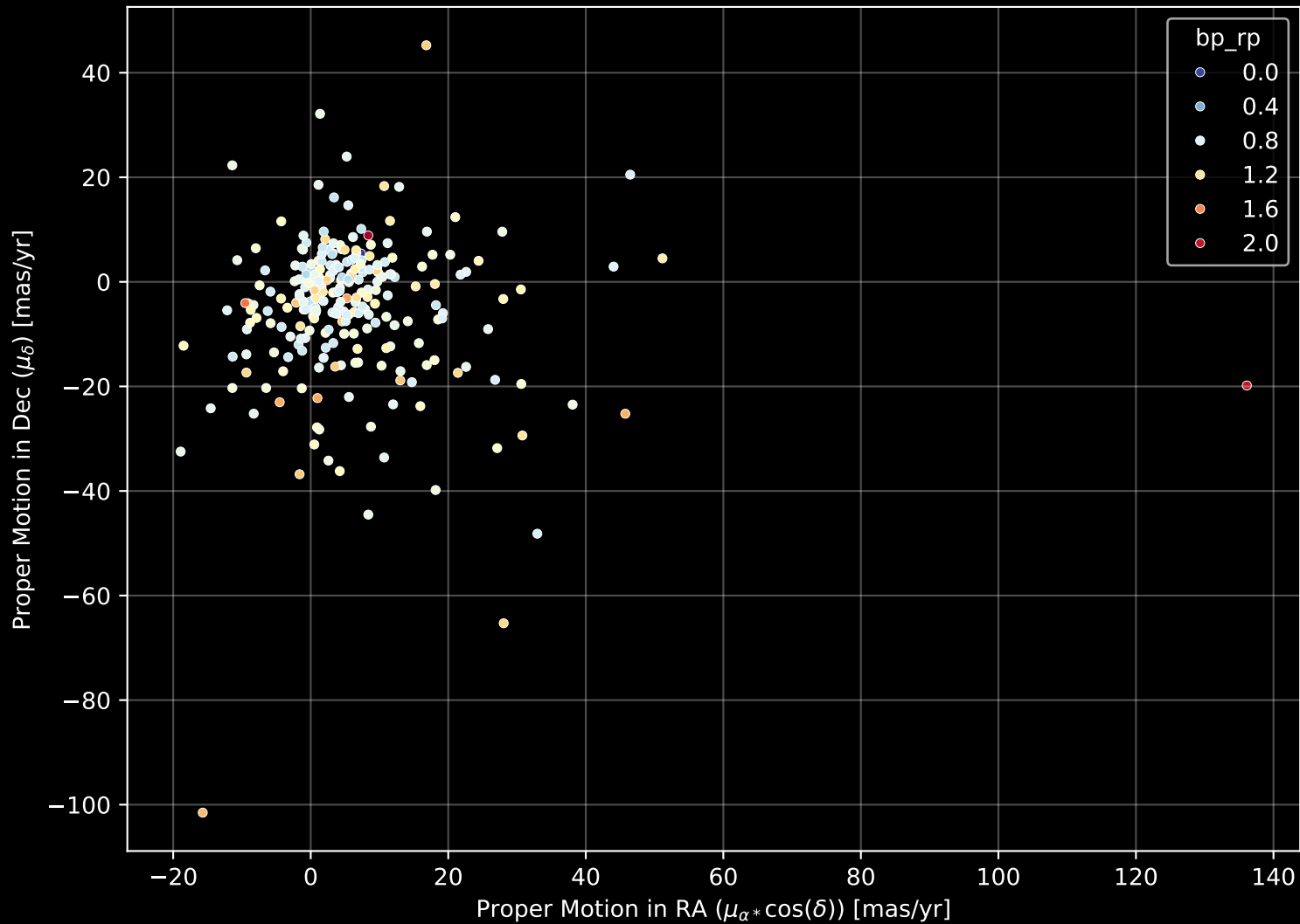
GALAH DR4 Field: [521] Proper Motion Diagram (n= 259)
