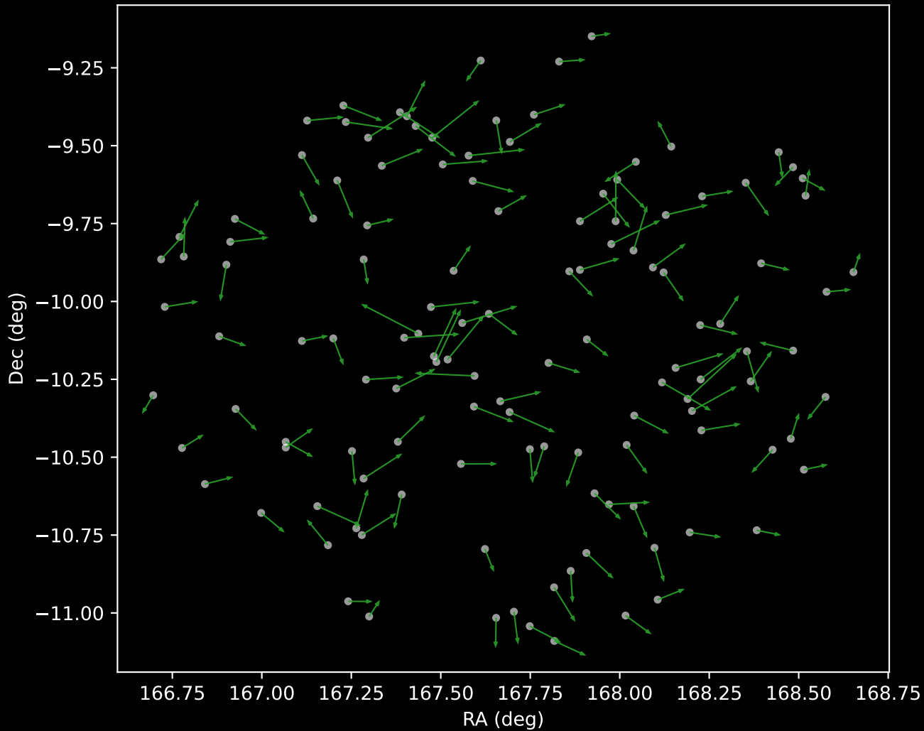
GALAH DR4 Cluster 4 Proper Motion Vectors (n=127)
