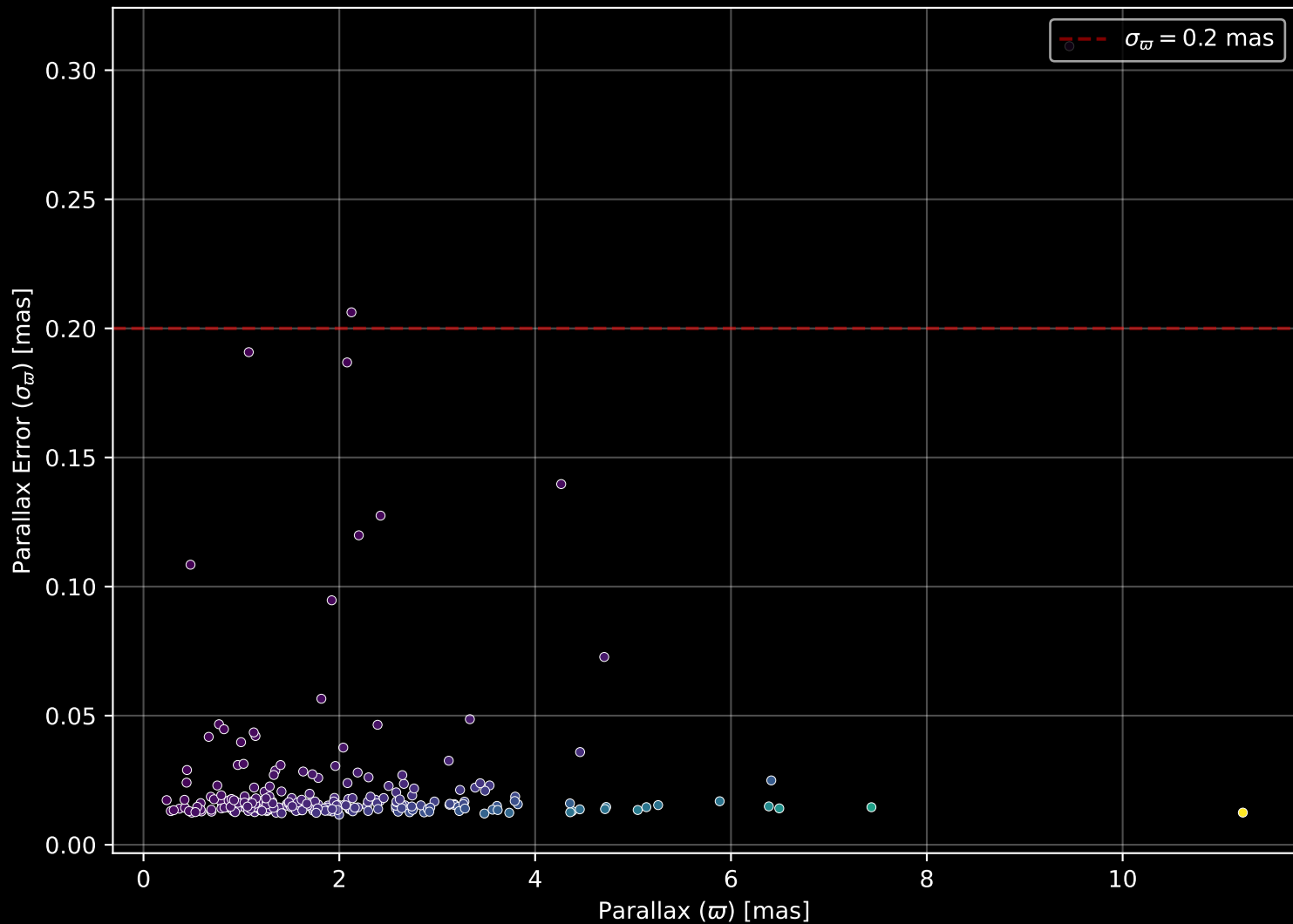
GALAH DR4 Field: [521] Parallax Quality (n= 259)
