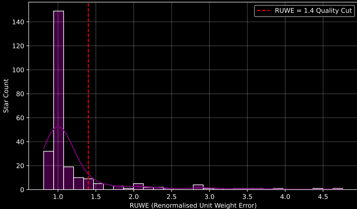
GALAH DR4 Field [521] RUWE Distribution (n= 250)
