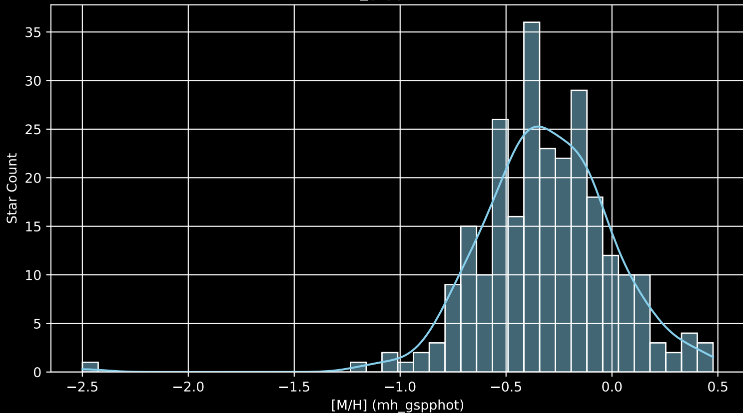
GALAH DR4 Field: [521] [M/H] (mh_gspphot) (n= 258)
