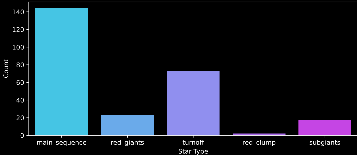
GALAH DR4 Field: [521] Count plot of Star Type
